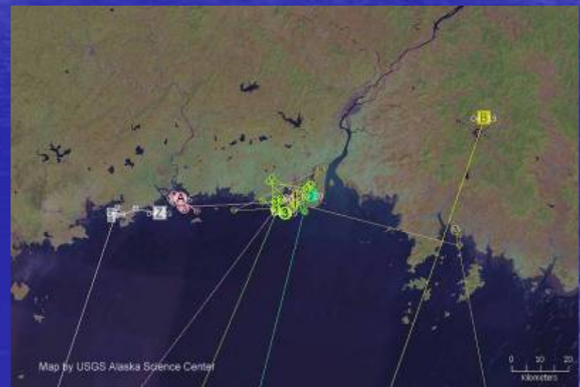
Satellite tracked shorebirds in 2007 and 2008
