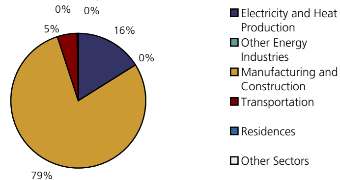
CO 2 Emissions by Sector, North Korea, 1999
