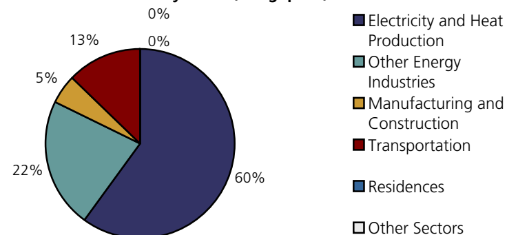
CO 2 Emissions by Sector, Singapore, 1999
